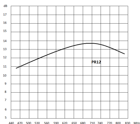
5G FILTER
