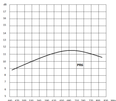
5G FILTER
